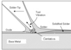
Figure 1 Illustration of cavitation during ultrasonic soldering.
